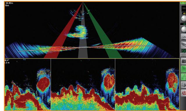
WMB-3230 Real-time acoustic polar and triple beam view
