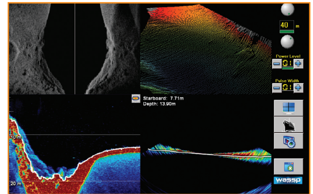
WMB-3250 Multi-functional display
