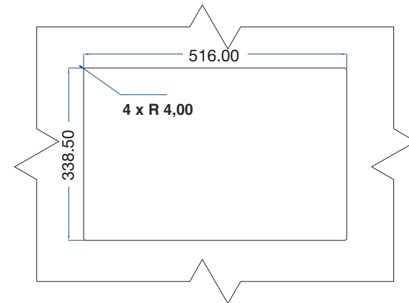
PANEL CUTOUT
